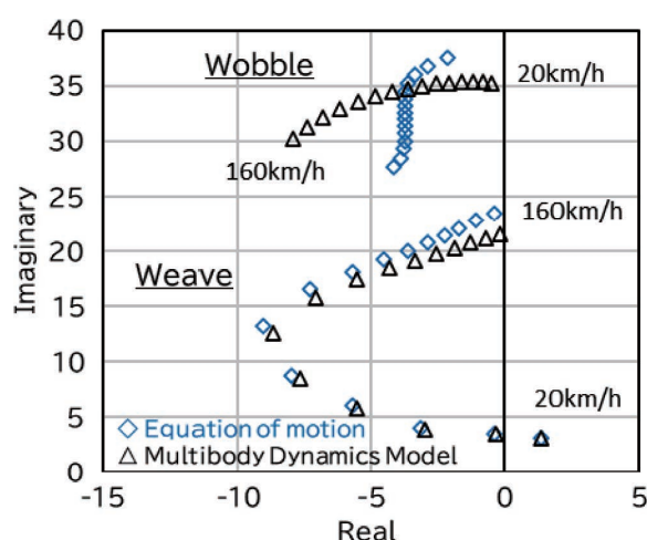
図3 Root Locus
