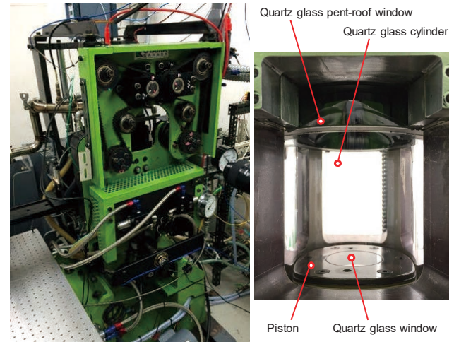
Fig. 1 Optical engine
