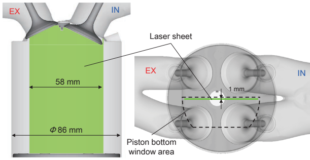
Fig. 4 Schematic of measurement range
