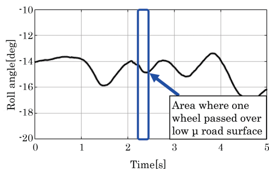
Fig.5 Roll Angle Measurement Data at Left Turn
