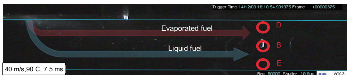
Fig.20 Passages of evaporated fuel and liquid fuel
