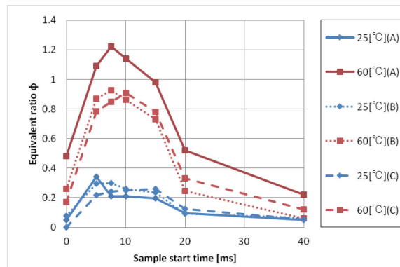
Fig.14 Equivalent ratio (n-heptane, 60 C)
