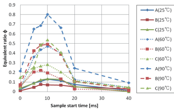
Fig.6 Equivalent ratio (n-heptane, 40 m/s)
