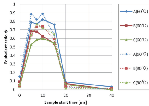
Fig.9 Equivalent ratio (i-pentane, 40 m/s)
