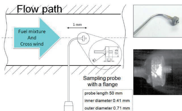
Fig.2 Gas sampling probe
