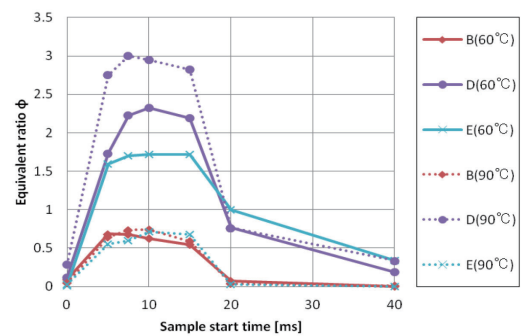
Fig.10 Equivalent ratio (i-pentane, 40 m/s)
