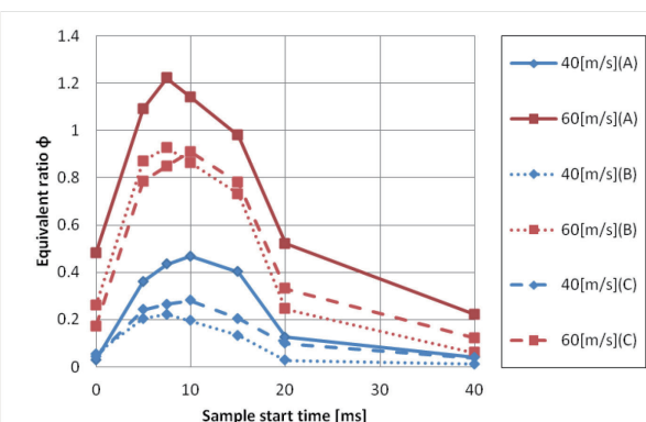
Fig.19 Equivalent ratio (n-heptane, 60 m/s)
