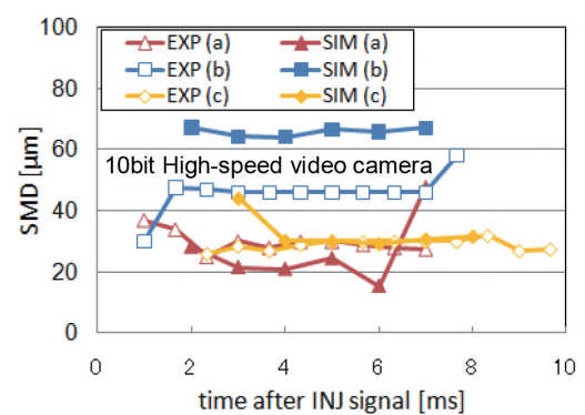
Fig.28 Comparison of SMD between calculation and measurement at three areas
