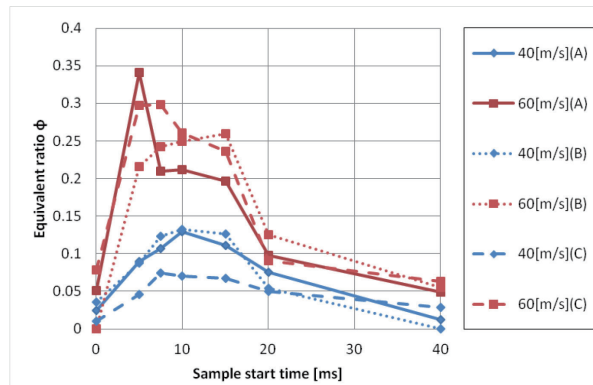
Fig.13 Equivalent ratio (n-heptane, 25 C)
