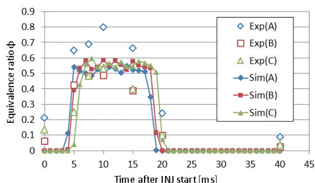
Fig.29 Comparison of equivalence ratio between calculation and measurement at three positions (n-heptane, 40 m/s, 90 C)
