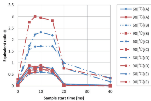
Fig.21 Equivalent ratio (i-pentane, 40 m/s)
