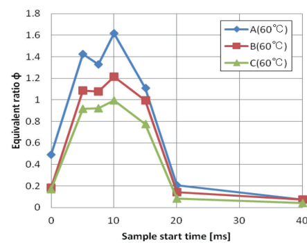
Fig.11 Equivalent ratio (i-pentane, 60 m/s)
