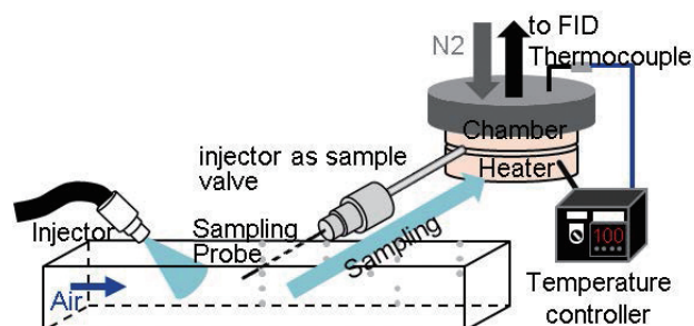
Fig.3 Schematics of gas sampling system
