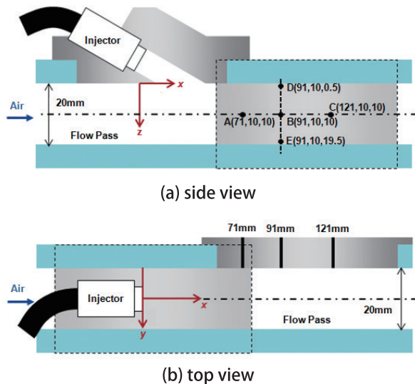
Fig.5 Measured points of gas sampling
