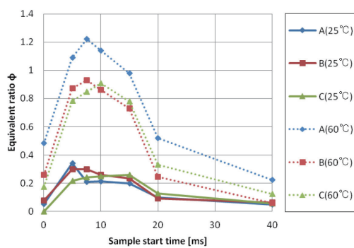
Fig.8 Equivalent ratio (n-heptane, 60 m/s)
