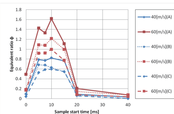
Fig.15 Equivalent ratio (i-pentane, 60 C)
