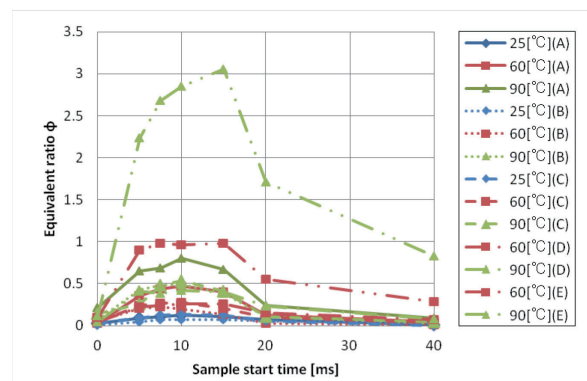
Fig.18 Equivalent ratio (n-heptane, 40 m/s)
