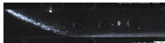
(b): n-heptane, 40 m/s, 60 C, 7.5 ms
