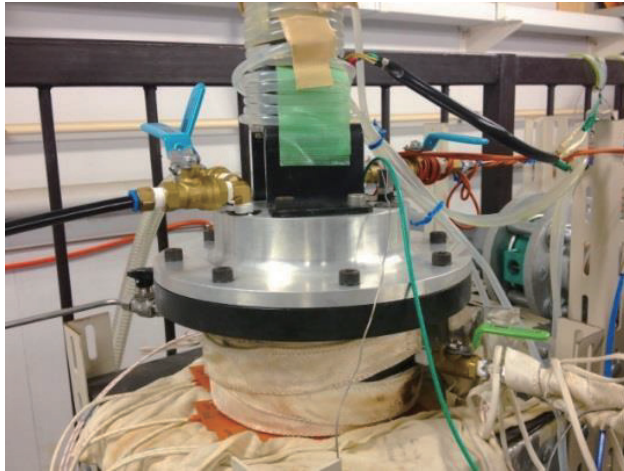
Fig.4 Picture of the sampled gas chamber
