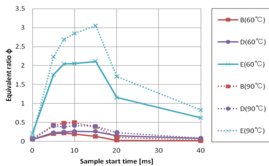
Fig.7 Equivalent ratio (n-heptane, 40 m/s)
