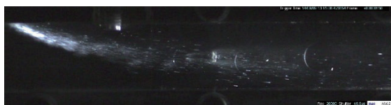
(a): n-heptane, 60 m/s, 25 C, 7.5 ms
