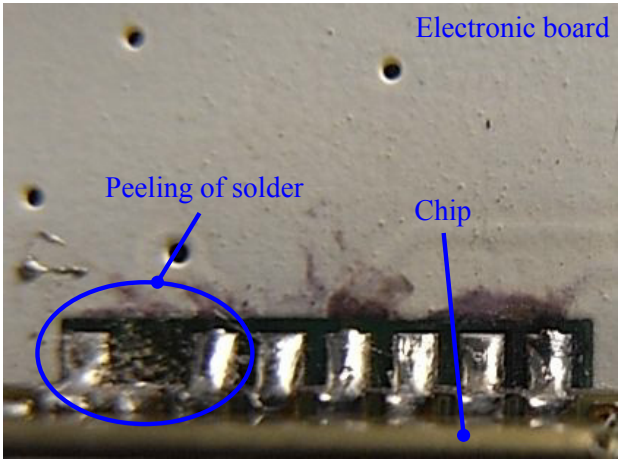
Figure 2: Component Damage Caused by Vibrations
