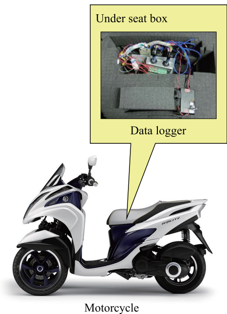
Figure 11: Example of Data Logger Mounting
