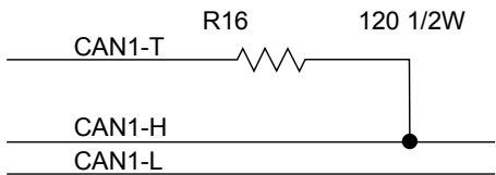
Figure 8: Terminal Connection of CAN Communication
