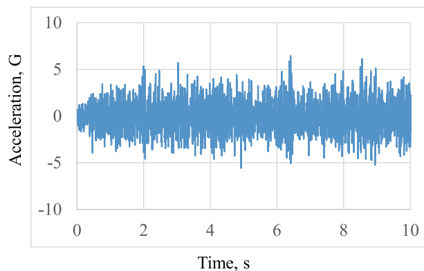
Figure 5: Acceleration under Seat
