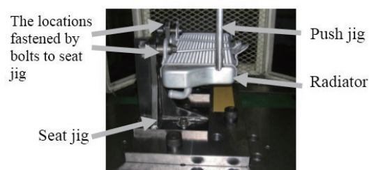
Figure 10: Radiator individual component strength test
