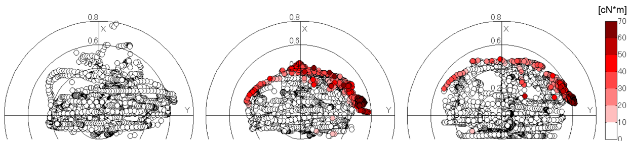
Figure 11 Plots of running state on friction ellipse. Left: without control, Center: PD control with friction ellipse of \mu_\alpha = 0.54 and \mu_\gamma = 0.5 , Right: PD control with friction ellipse of \mu_\alpha = 0.648 and \mu_\gamma = 0.6 , ( \mu_\alpha : longitudinal axis, \mu_\gamma : lateral axis).
