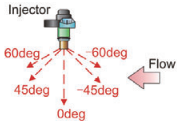
Fig. 2 Definition of injection direction to the flow
