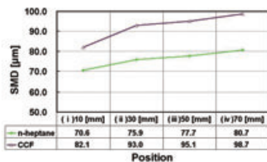
Fig. 9 SMD values along the spray axis
