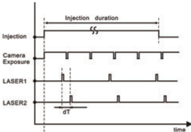
Fig. 4 Timing chart for experiments
