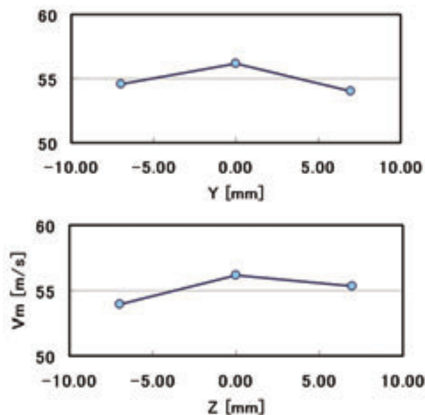
Fig. 6 LDV measured mean velocity
