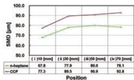
Fig. 9 SMD values along the spray axis
