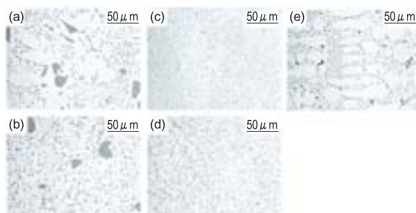
Fig.5 Microstructures of (a) AFC12 before forging, (b) AFC12 after forging, (c) AFP10 after forging, (d) AFP20 after forging and (e) AC8A as cast
