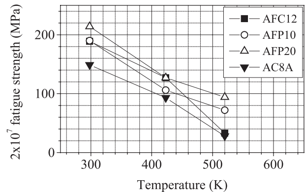
Fig.13 Fatigue strength at various temperatures
