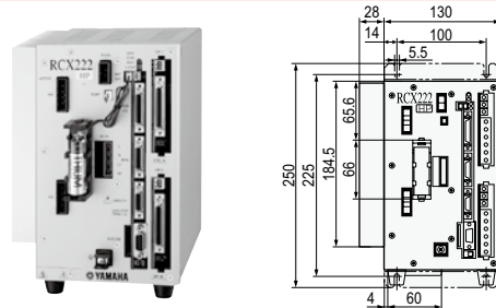
RCX222HP Dimensions
