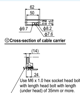
Detail of section C
