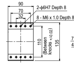
Detail section A
