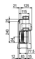
② Cross-section of cable carrier
